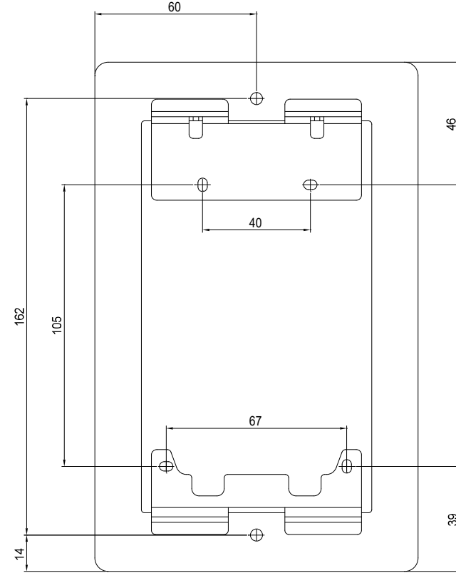
4 BACK VIEW
