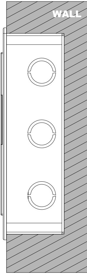
3 SIDE VIEW: INTERCOM PANEL ON WALL
