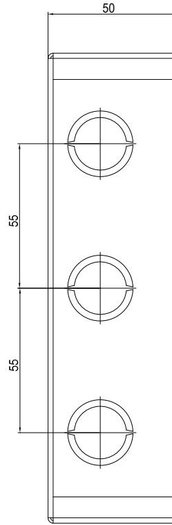
3 LEFT VIEW
