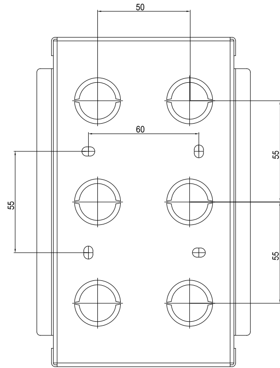
4 BACK VIEW
