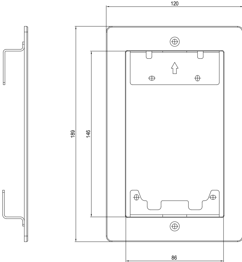
1 FRONT VIEW
