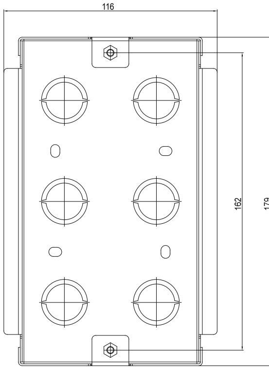
1 FRONT VIEW
